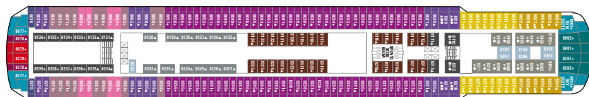
Deck 8
